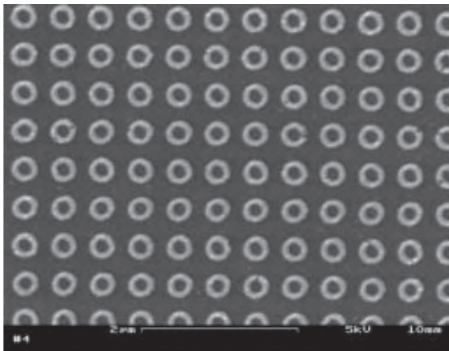
Figure 2: Silver nanorings.
