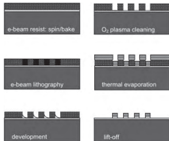
Figure 1: Nanofabrication protocol.
