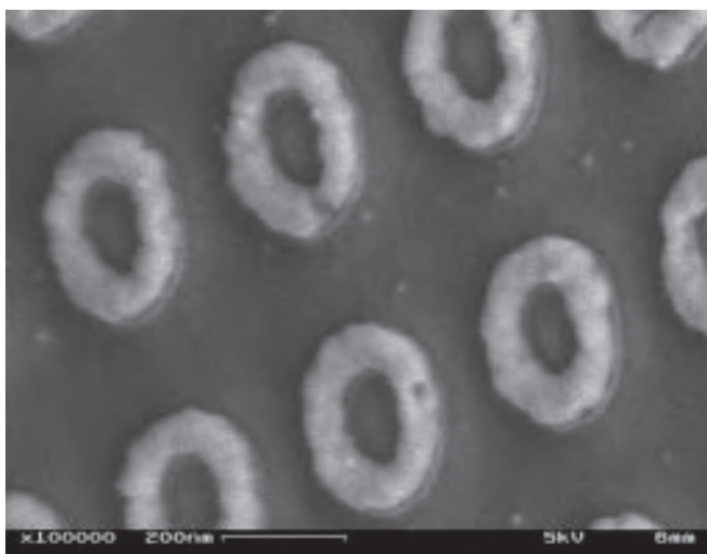
Figure 3: Tilted view of silver nanorings.
